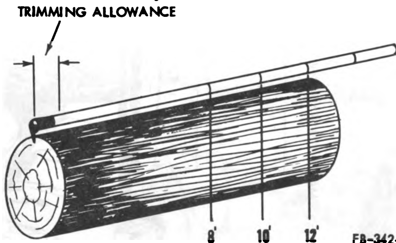
Figure 6-4. A log measuring pole.
